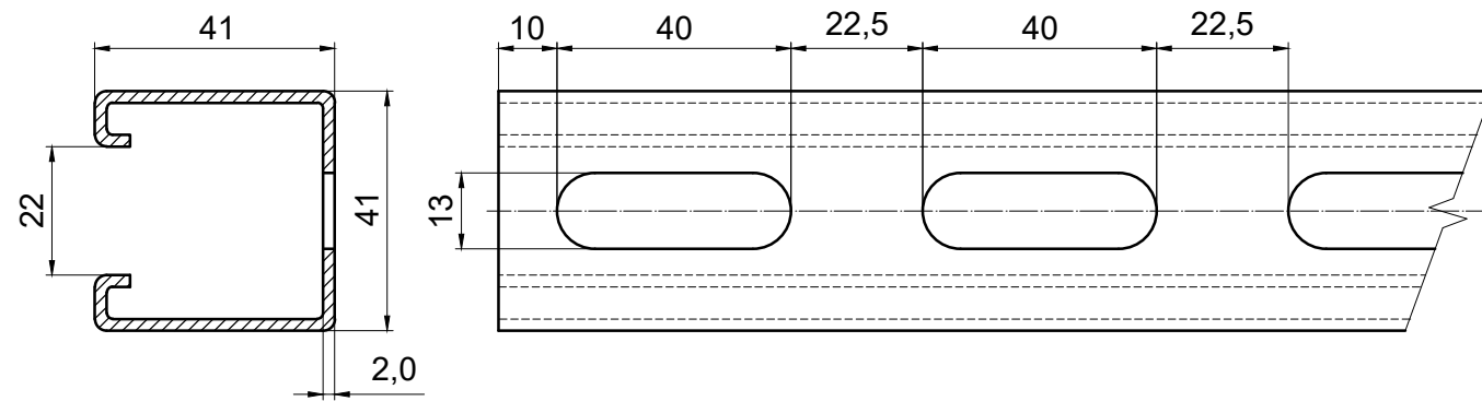
ST41x41x2,0mm
