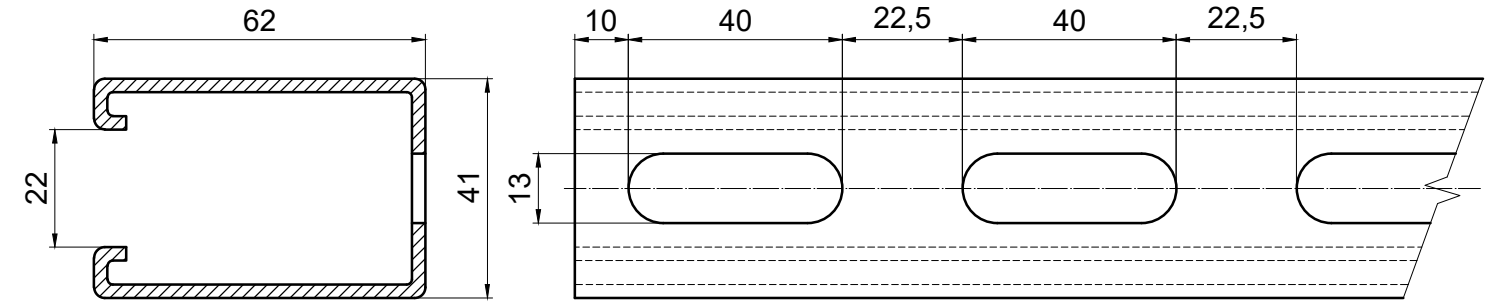
ST41x62x2,5mm
