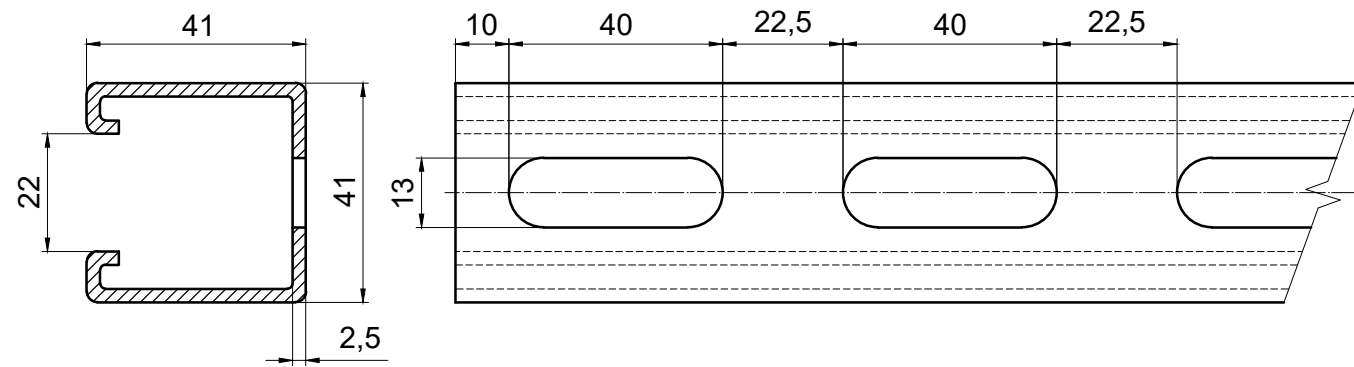
ST41x41x2,5mm
