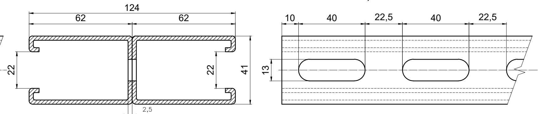
ST2x41x62x2,5mm
