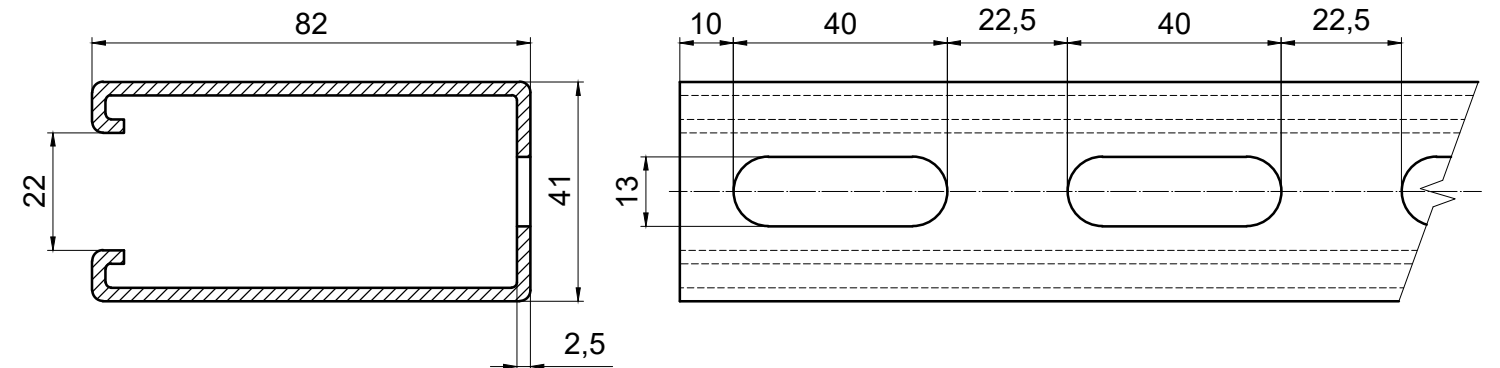
ST41x82x2,5mm
