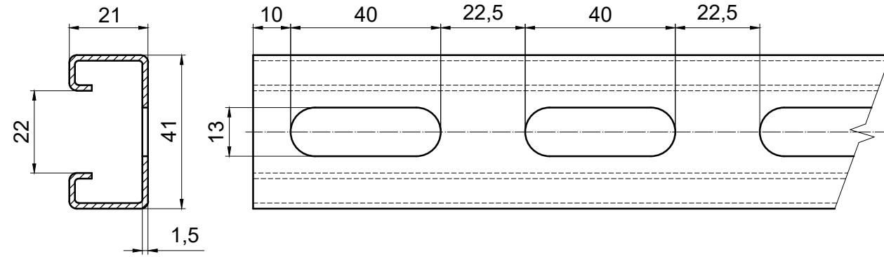
ST41x21x1,5mm
