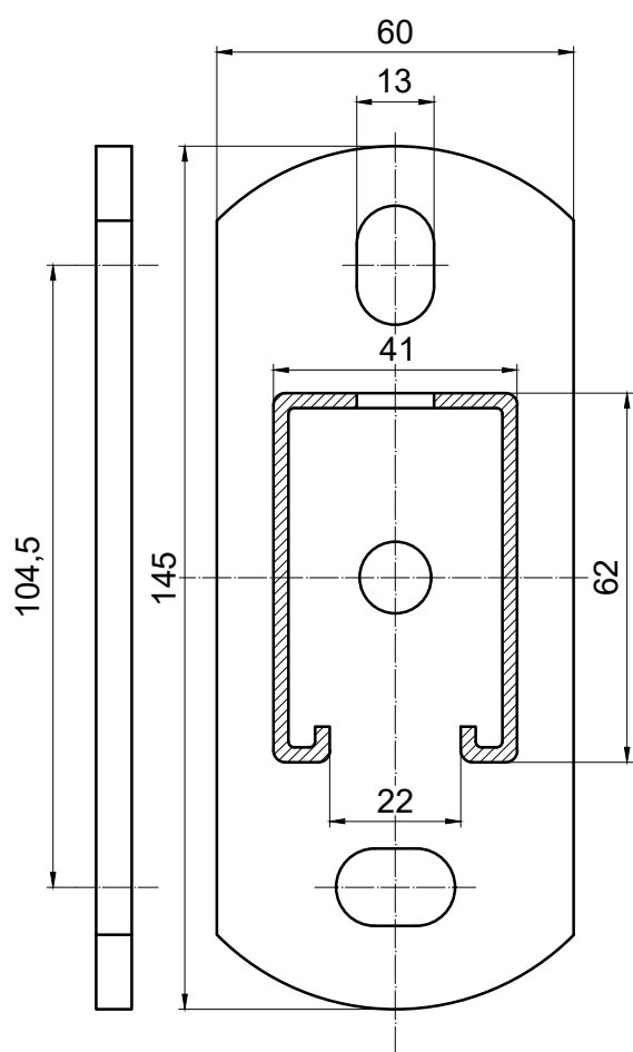
ST41x62x2,5mm
