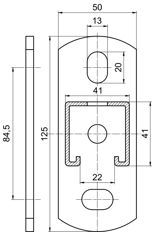
ST41x41x2,5mm
