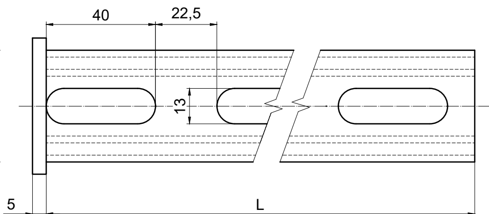
ST41x41x2,5mm
