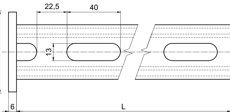
ST41x62x2,5mm
